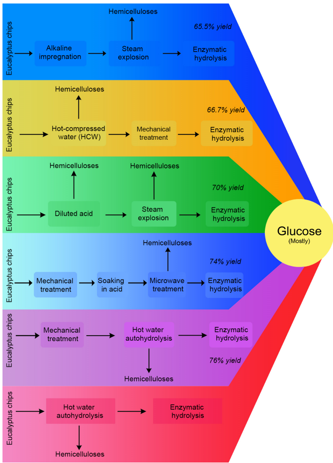
Fig.6. Schematic representation of reported pretreatments on eucalyptus producing medium enzymatic hydrolysis yields.
