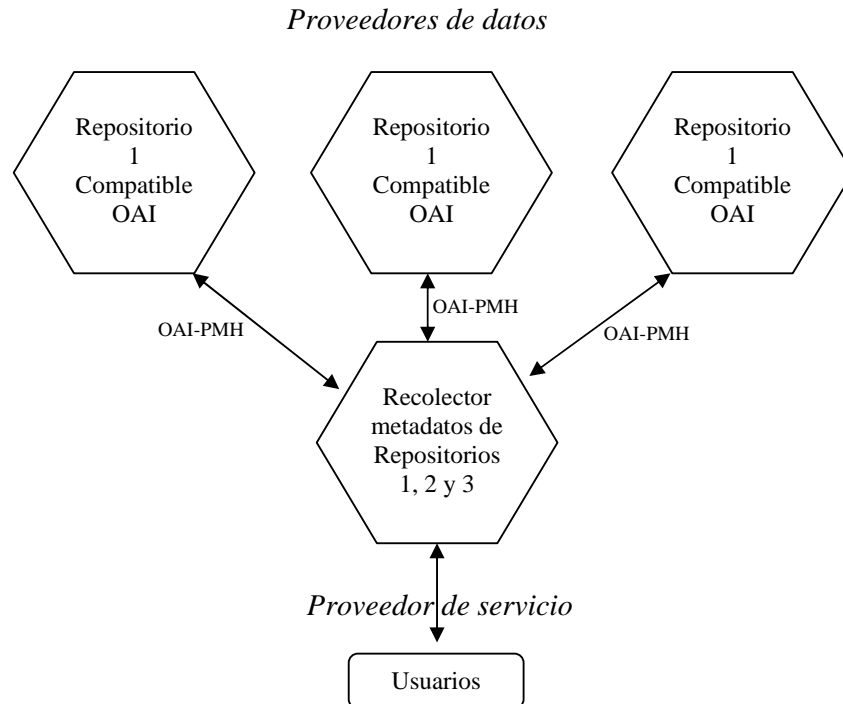
Fig. 1: Protocolo OAI-PMH
